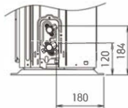
Side view (Bulb part)
