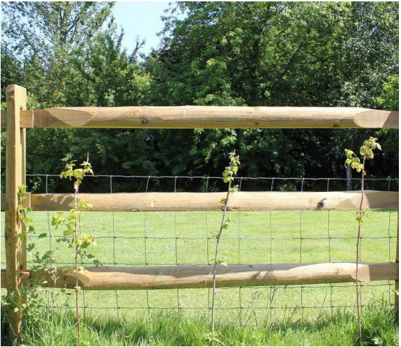
Timber post and rail fence with heavy duty dog proof mesh
