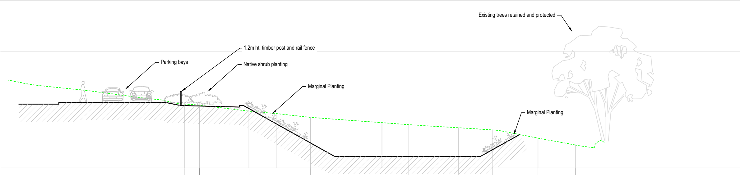
AA Typical Section AA
