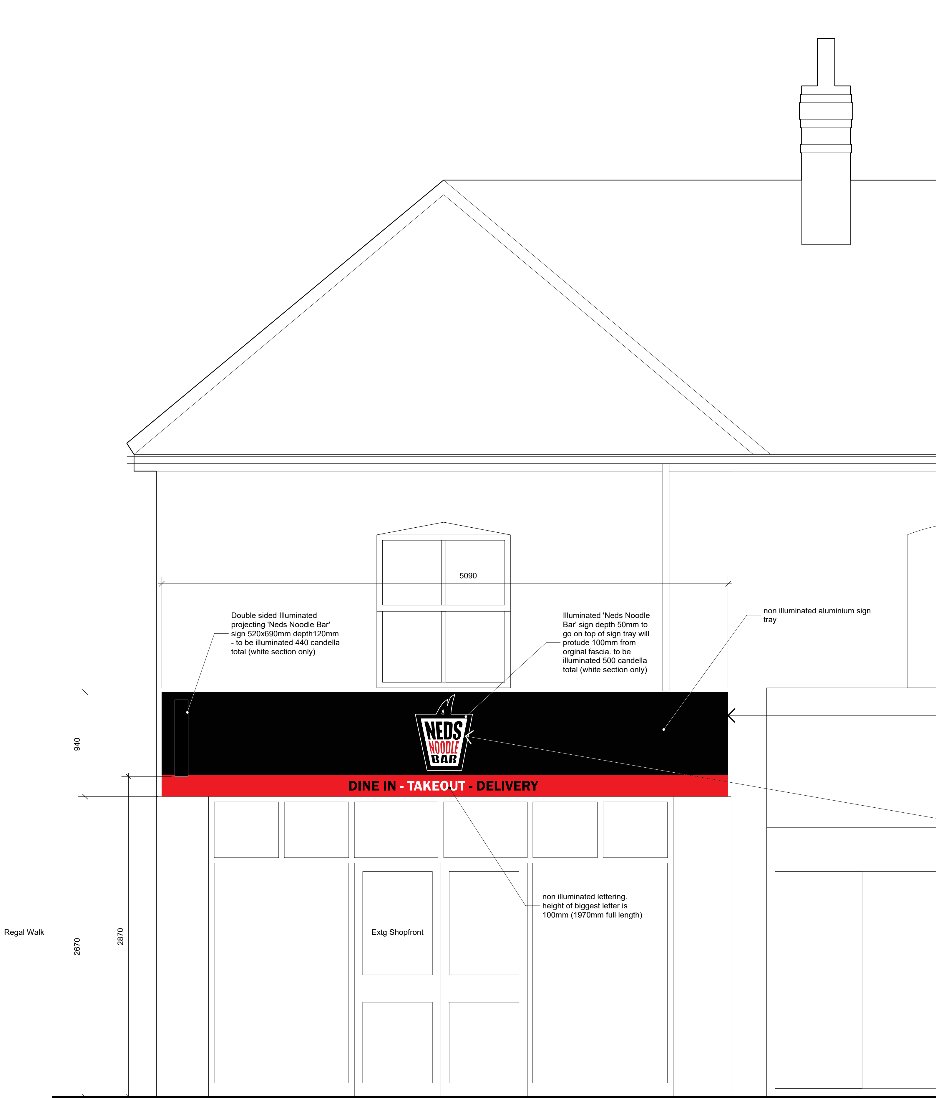
Front Elevation as Proposed 1:20 @ A1
