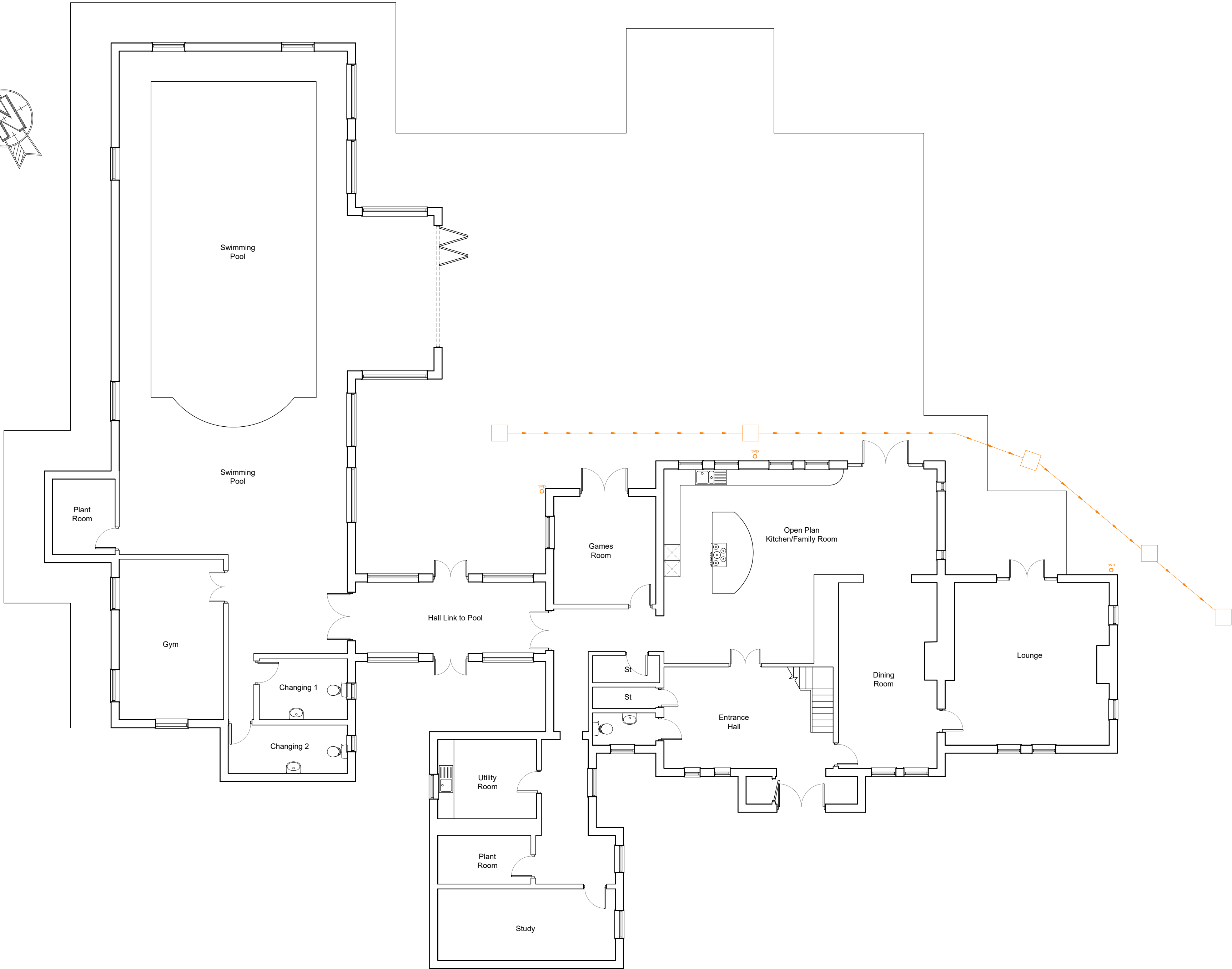
Existing Ground Floor - 1:100
