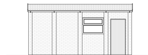
SIDE (SOUTH) ELEVATION
