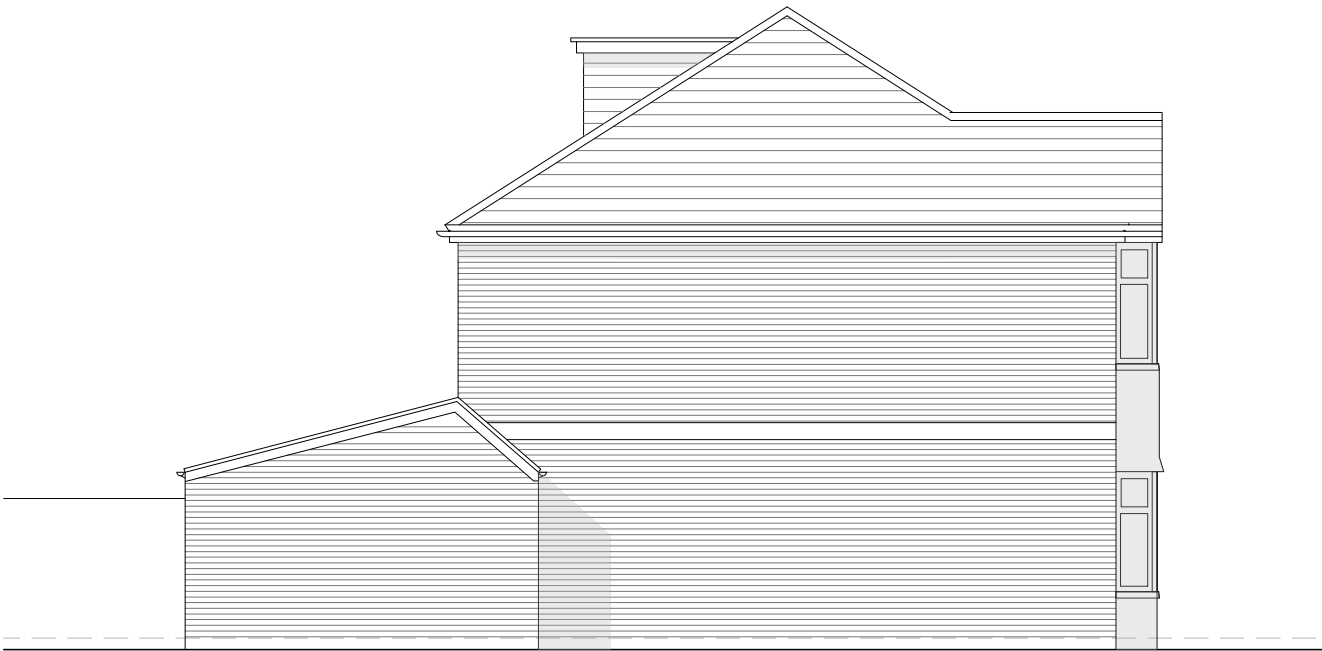
SIDE ELEVATION (SOUTH FACING)
