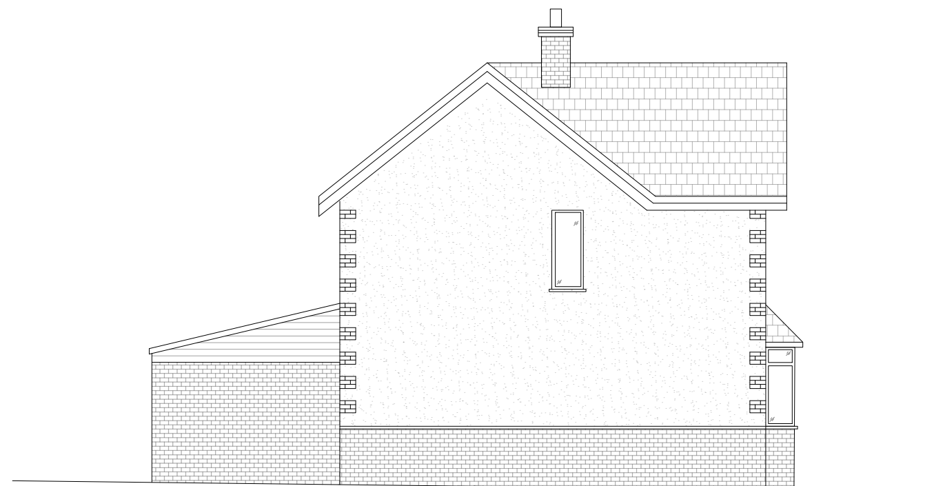
Existing Southwest Elevation 1:100 @A3
