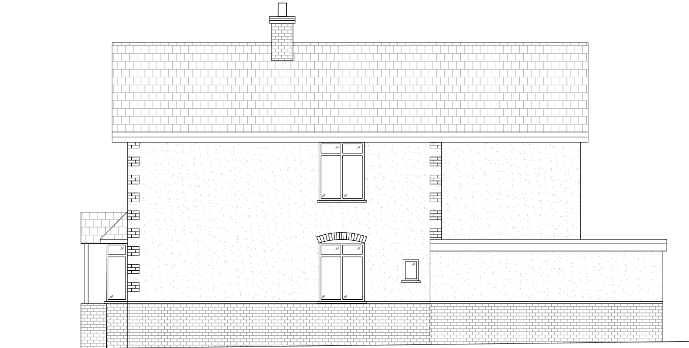
Proposed Northeast Elevation 1:100 @A3
