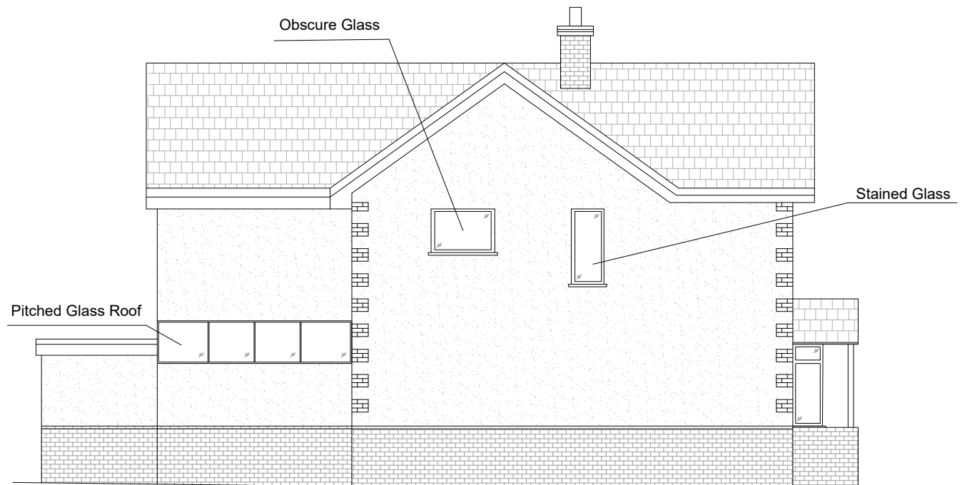
Proposed Southwest Elevation 1:100 @A3
