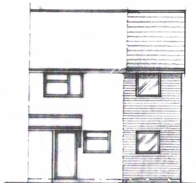
FRONT 1:100
