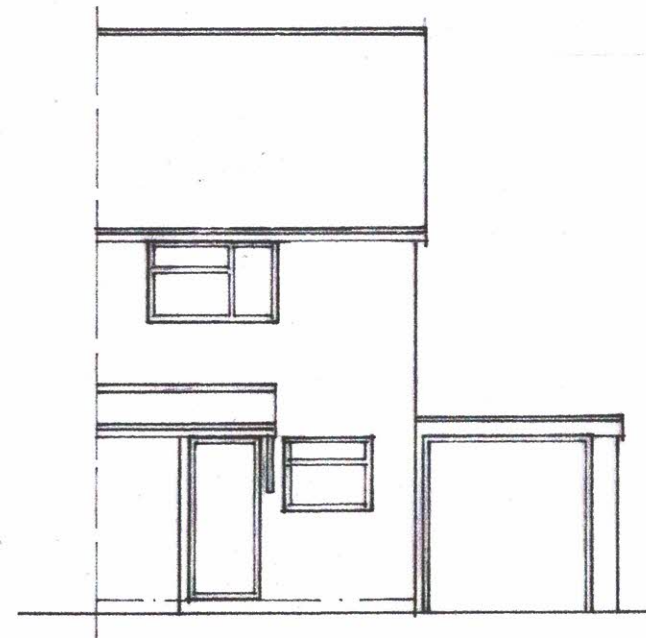
FRONT 1:100
