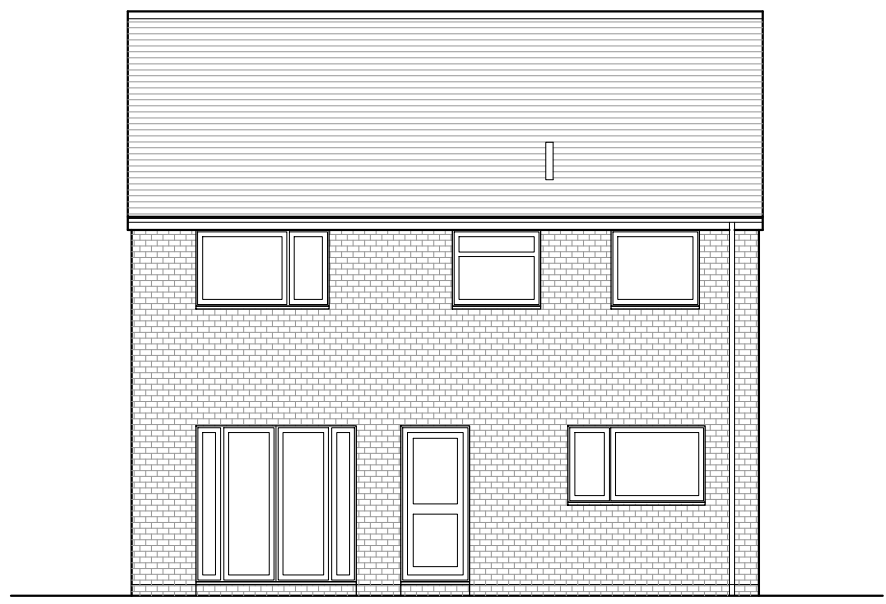
South-West (Rear) Elevation - As Existing
