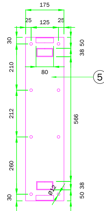
Base Plate: Front Elevation scale 1:10
