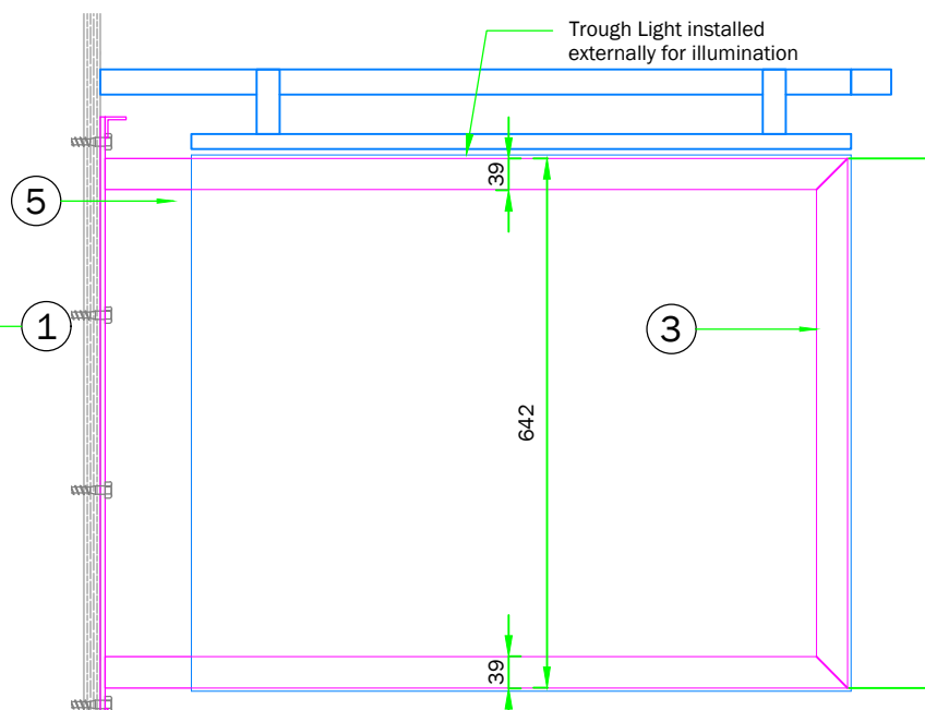
Framework: Front Elevation scale 1:10
