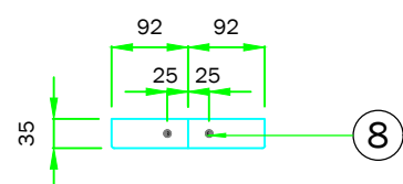
Shroud: Plan View scale 1:12
