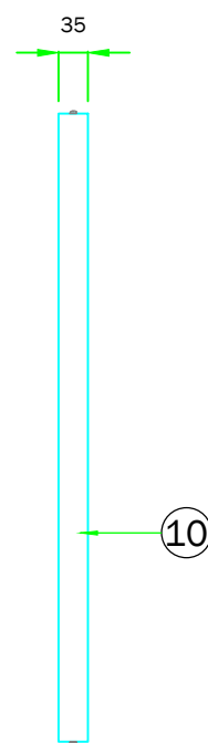
Shroud: End Elevation scale 1:10
