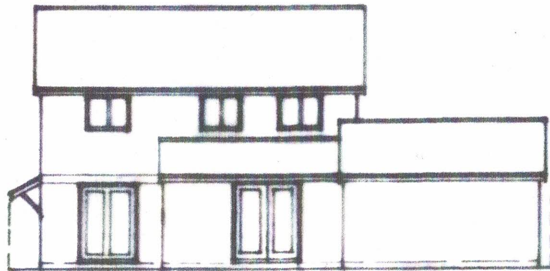
REAR (EAST)
