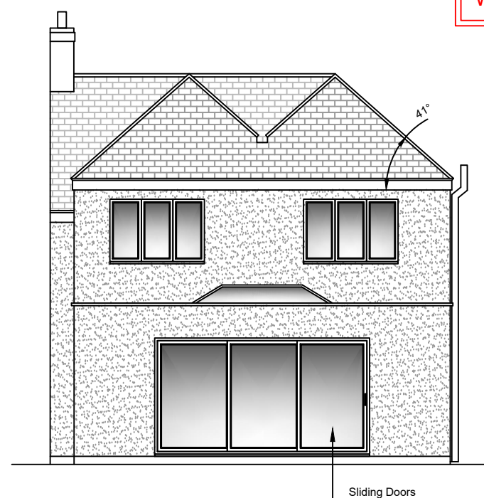
Rear Elevation
