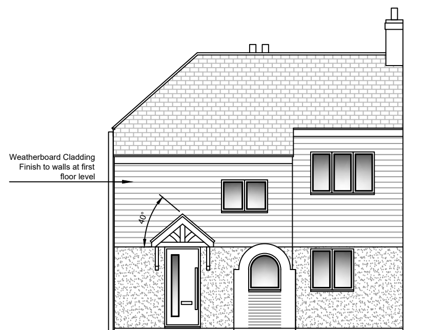
Front Elevation
