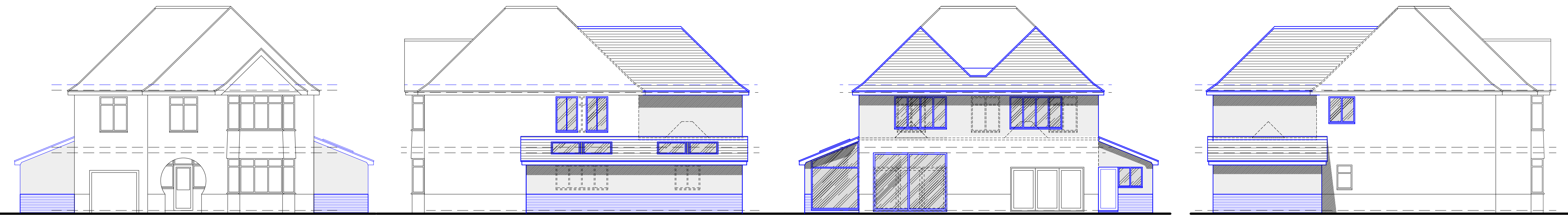
Proposed Front Elevation 1:100
