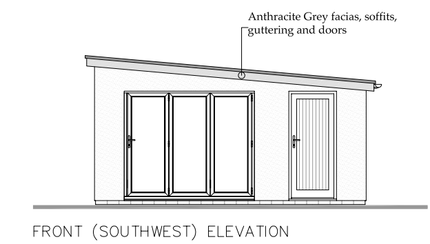
FRONT (SOUTHWEST) ELEVATION
