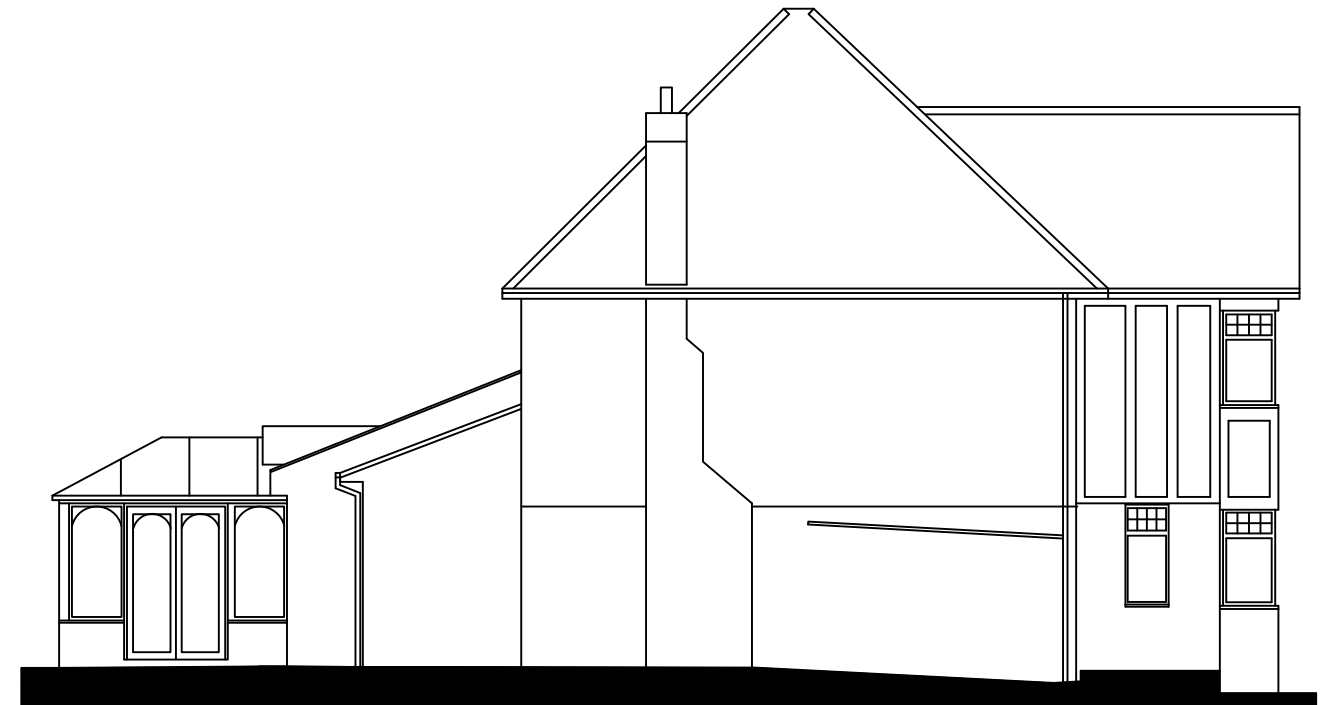
SOUTH ELEVATION | EXISTING 0m 1.0m 2.5m 5.0m 1:100
