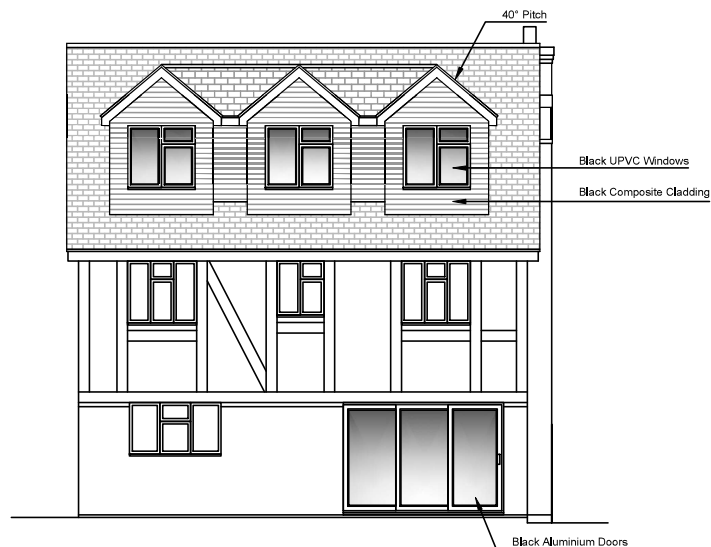
Rear Elevation
