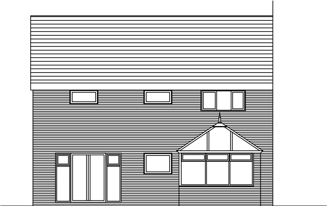
Rear Elevation
