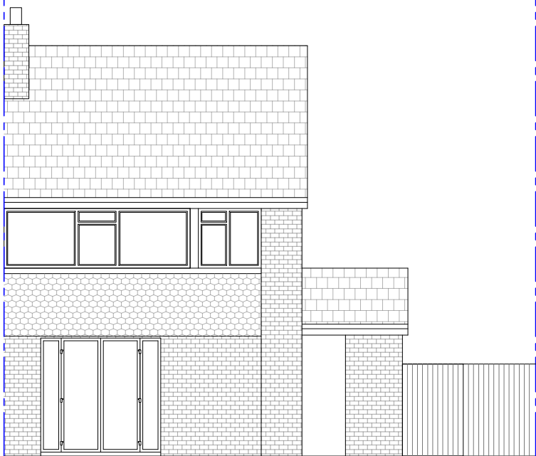
Existing Rear Elevation 1:100 @A3
