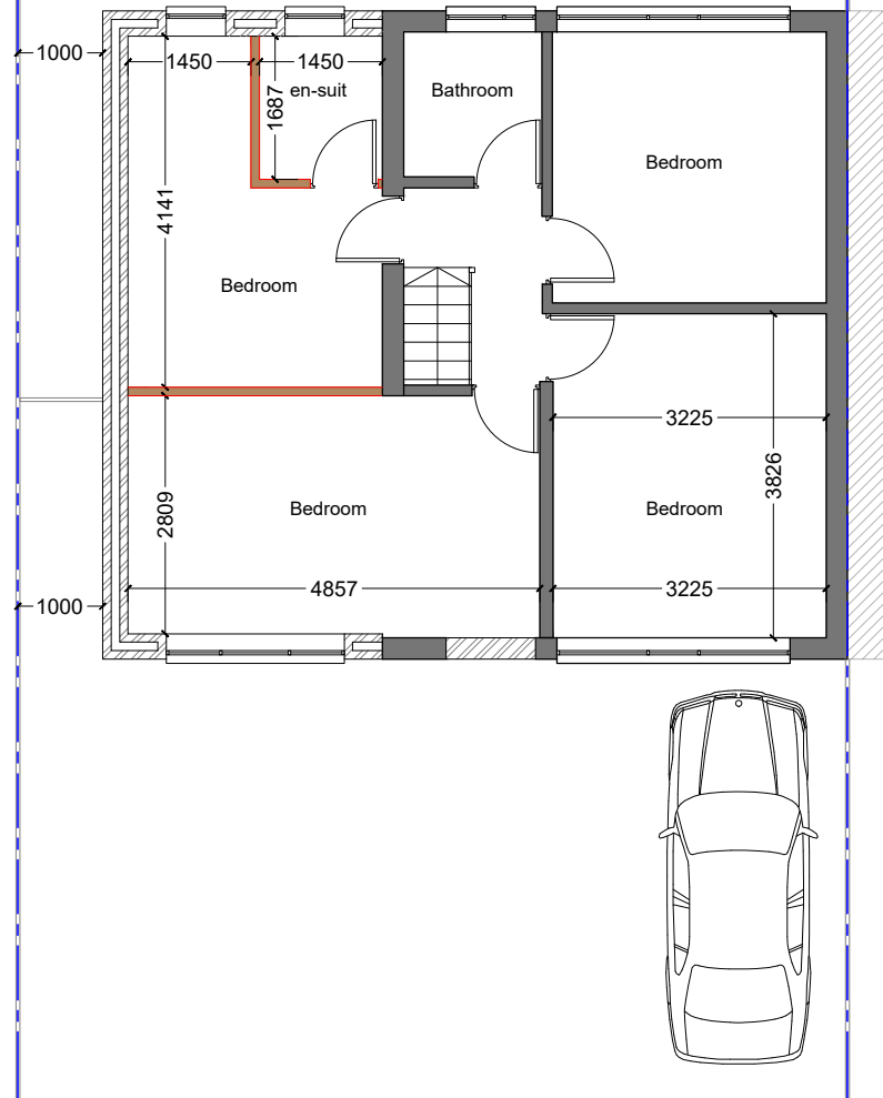
Proposed First Floor Plan 1:100 @A3
