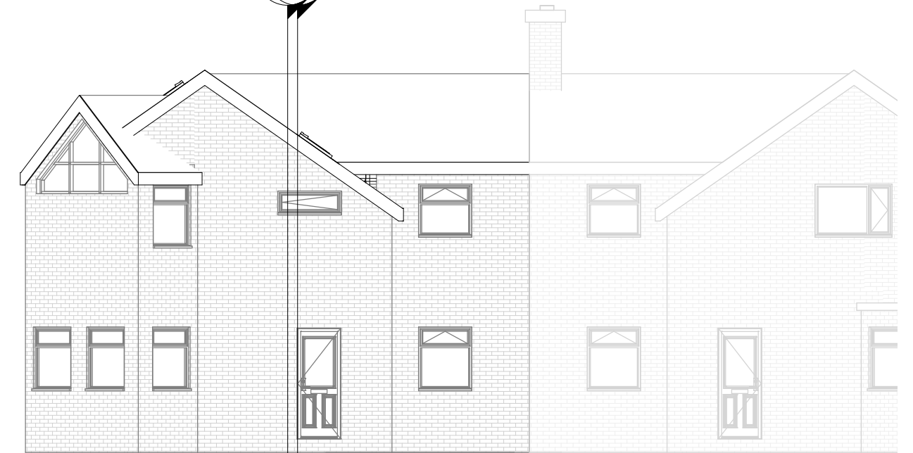
Proposed Elevation-Front
