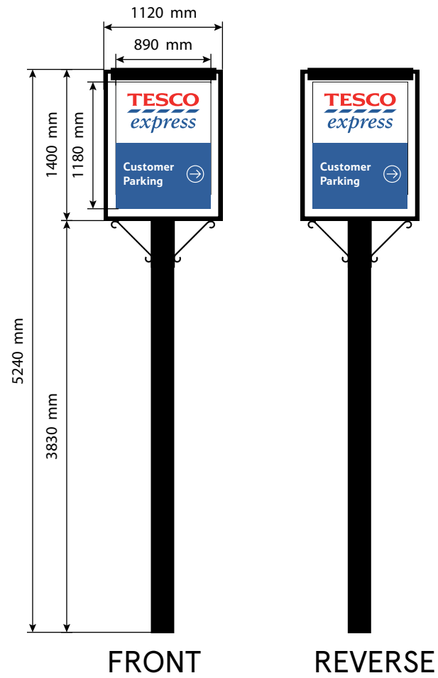
SIGN 20 Proposed New Gantry sign SIZE :1120X5240mm Existing externally illuminated gantry sign to be modified to latest design standards.
