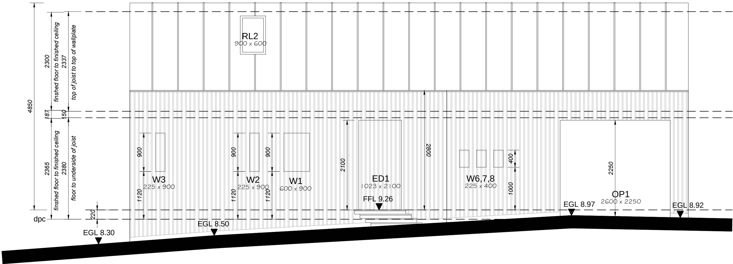
East Elevation
