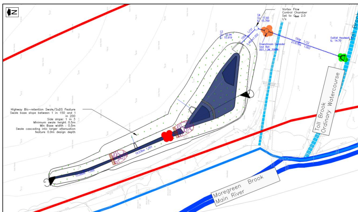
Figure 2.4 Southern Bio-retention Swale Monitoring Locations (from Drawing G277/27 Rev B)
