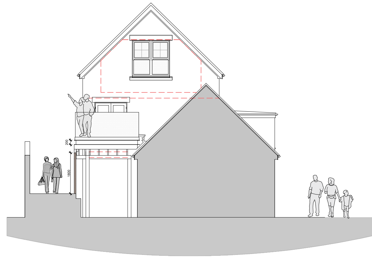
PROPOSED BACK ELEVATION (EAST)
