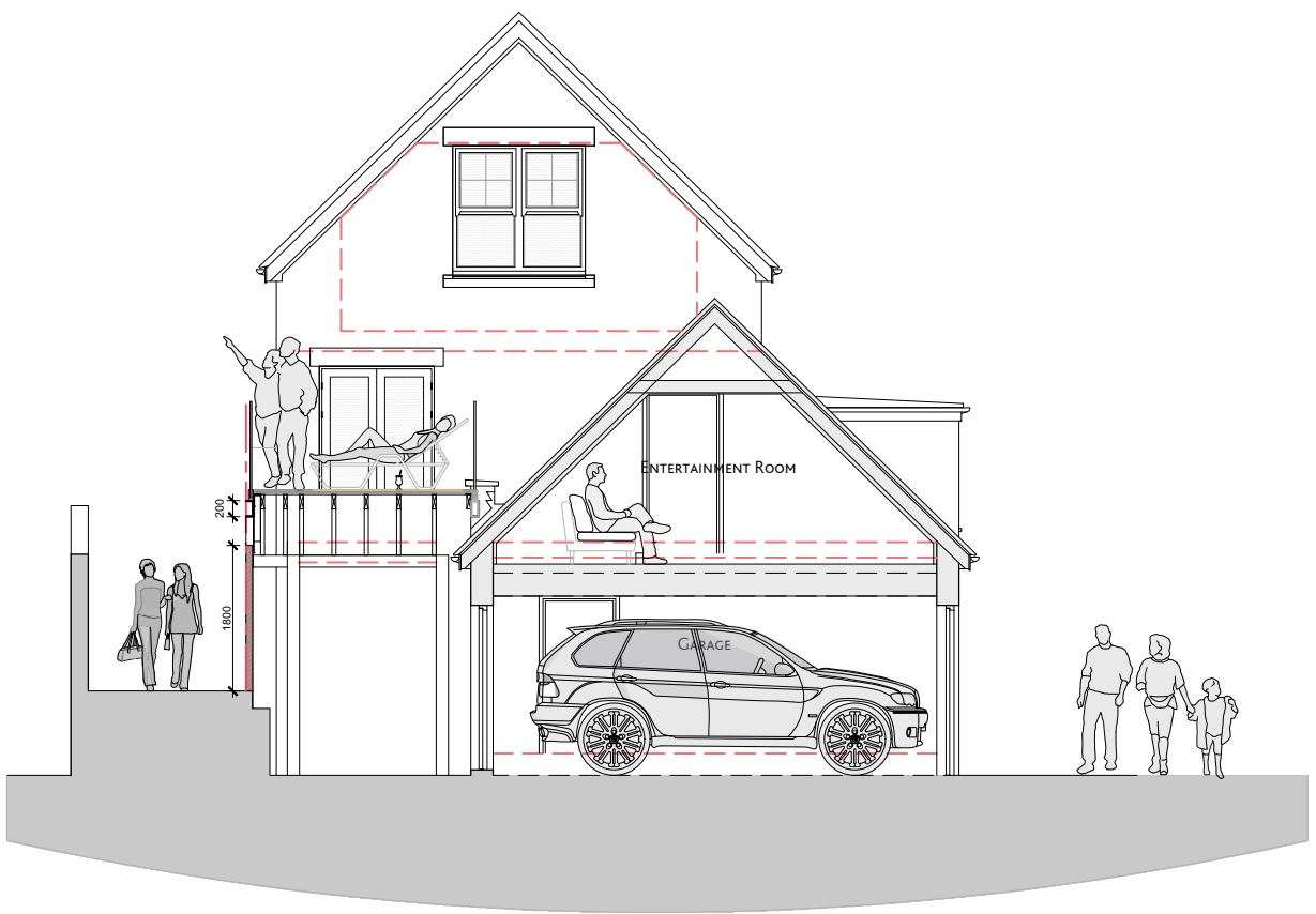
PROPOSED SECTION / ELEVATION (EAST) (FURTHEST FROM HOUSE)
