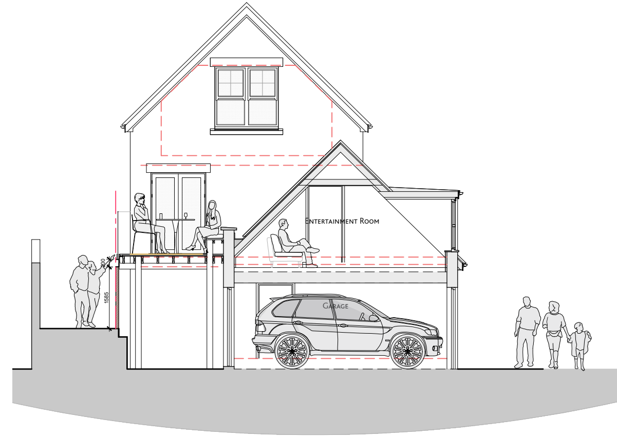
PROPOSED BALCONY SECTION (NEAREST HOUSE)
