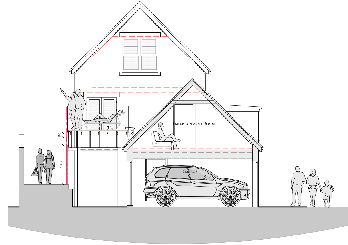
PROPOSED BALCONY SECTION (FURTHEST FROM HOUSE)
