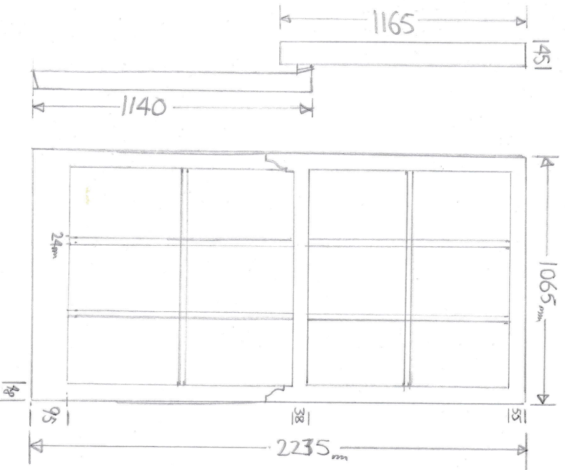
BACK ELEVATION
