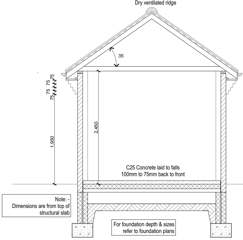
Section B-B | 1:50
