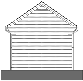
Rear Elevation | 1:100
