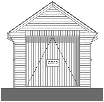
Front Elevation | 1:100
