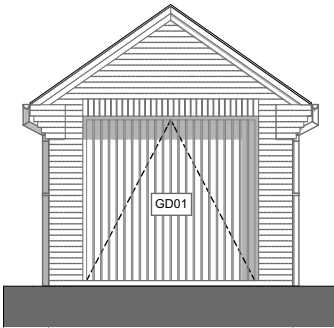
Front Elevation | 1:100
