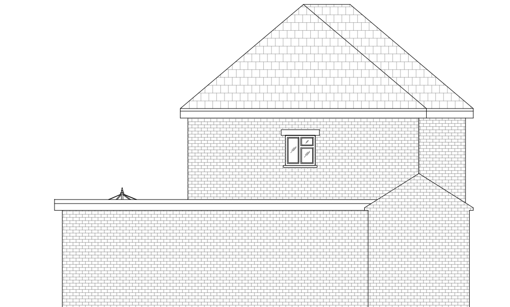
Existing East Elevation 1:100 @A3
