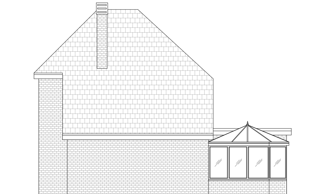
Existing West Elevation 1:100 @A3
