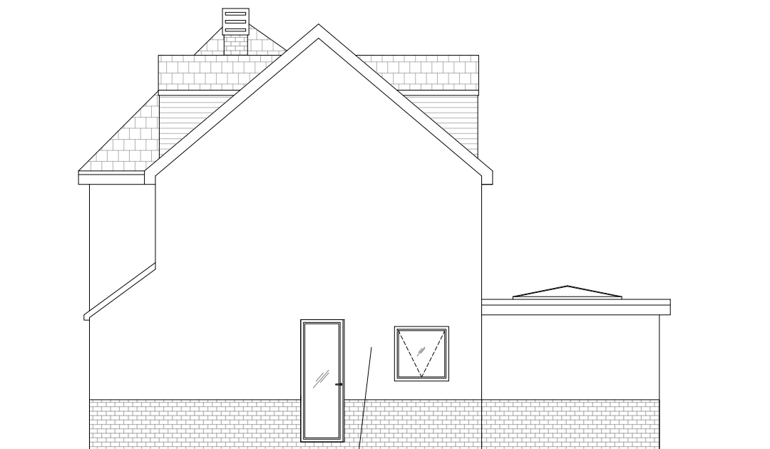
Proposed West Elevation 1:100 @A3
