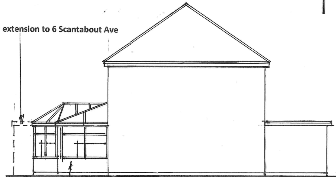
SIDE ELEVATION - EXISTING
