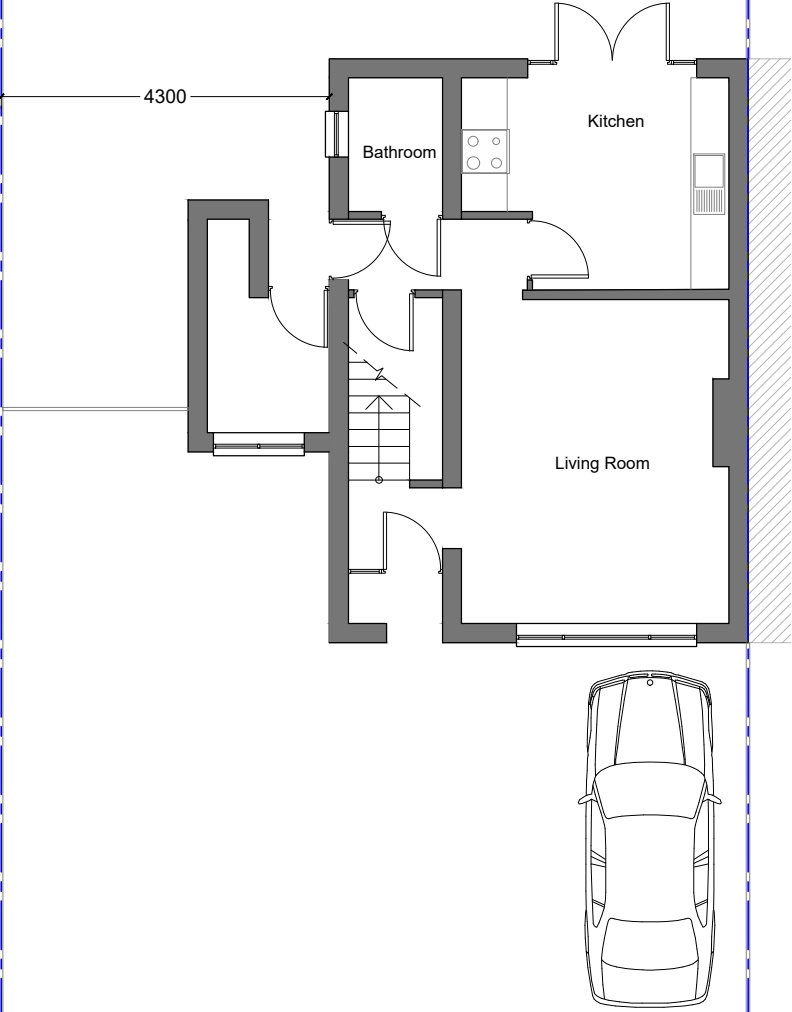
Existing Ground Floor Plan 1:100 @A3
