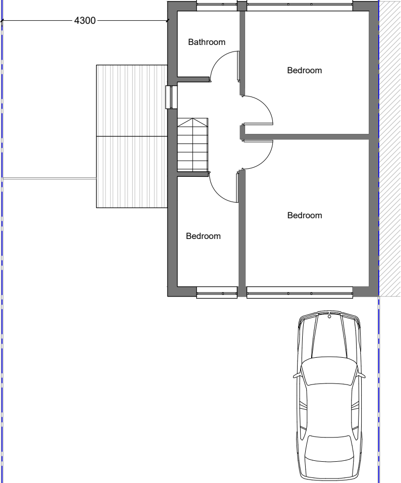
Existing First Floor Plan 1:100 @A3
