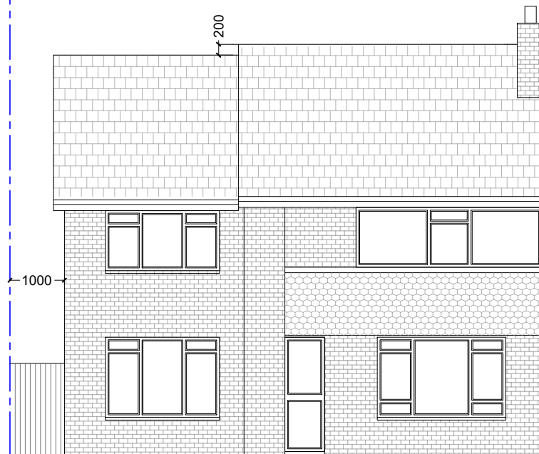
Proposed Front Elevation 1:100 @A3
