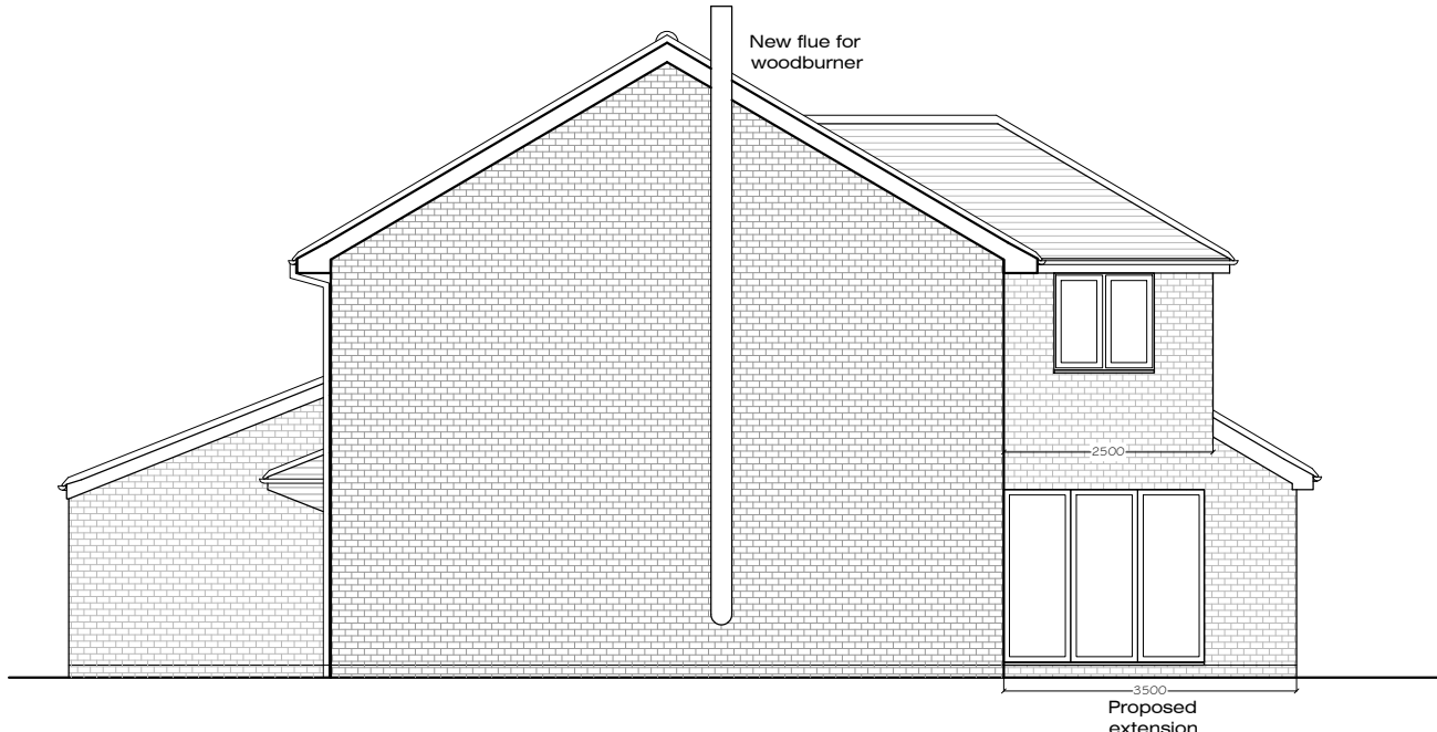
North-West (Side) Elevation - As Proposed
