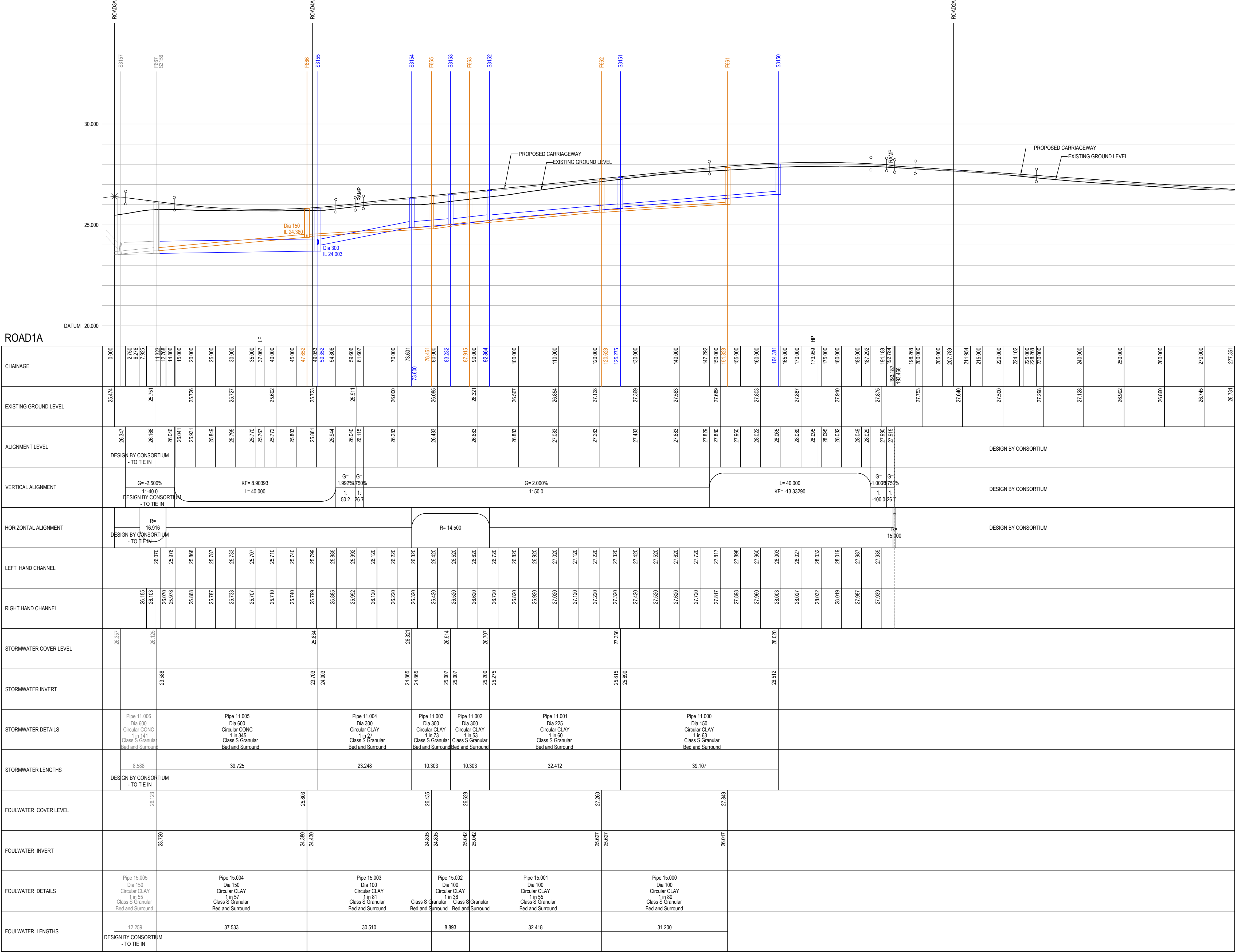
SECTION ROAD 1A SCALE H:1:500 V:1:100
