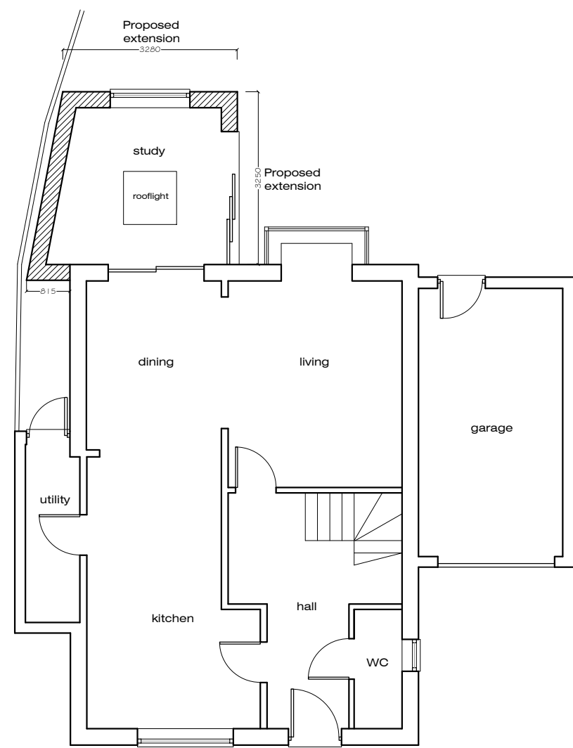
Ground Floor Plan - As Proposed
