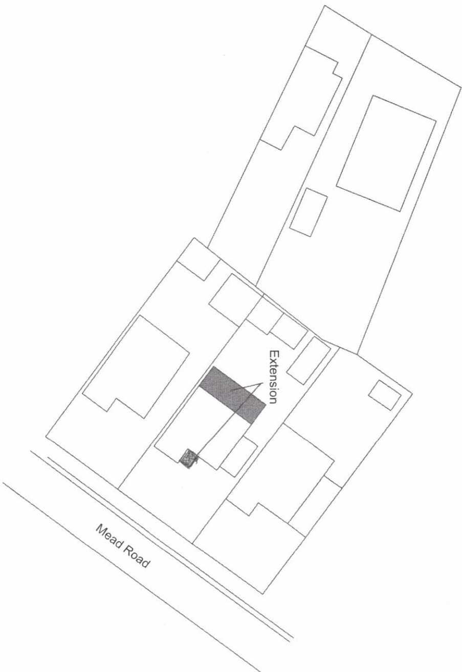
Block Plan 1:500
