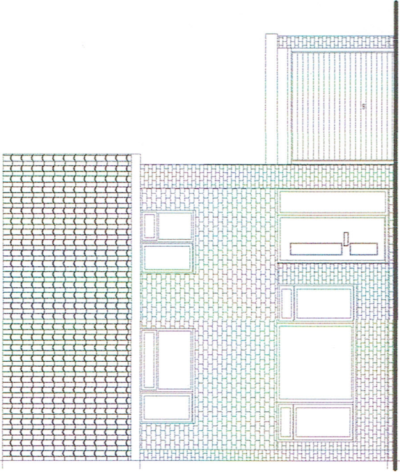
Front Elevation
