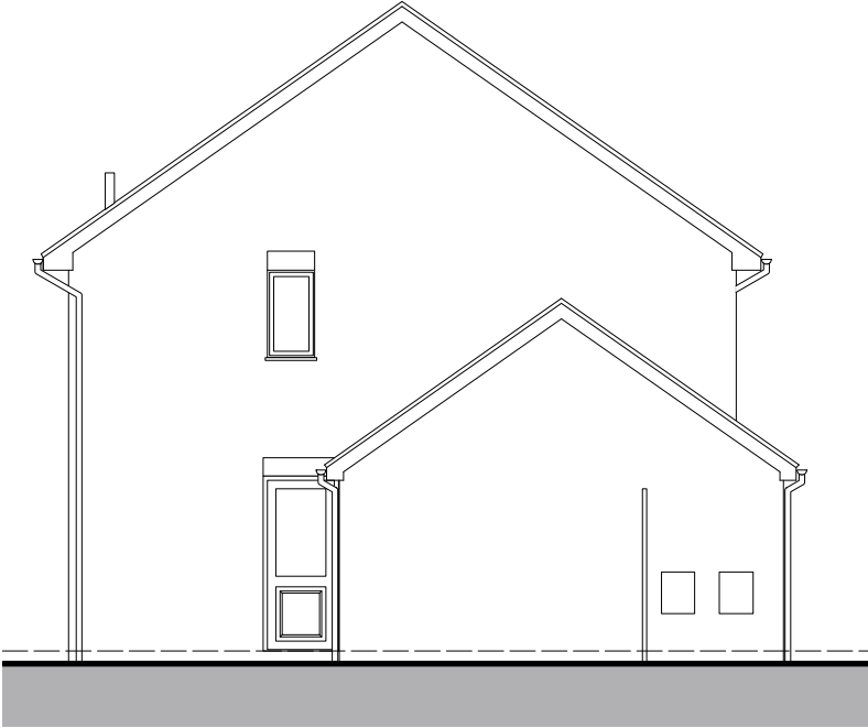
EXISTING SOUTH EAST ELEVATION 1:100
