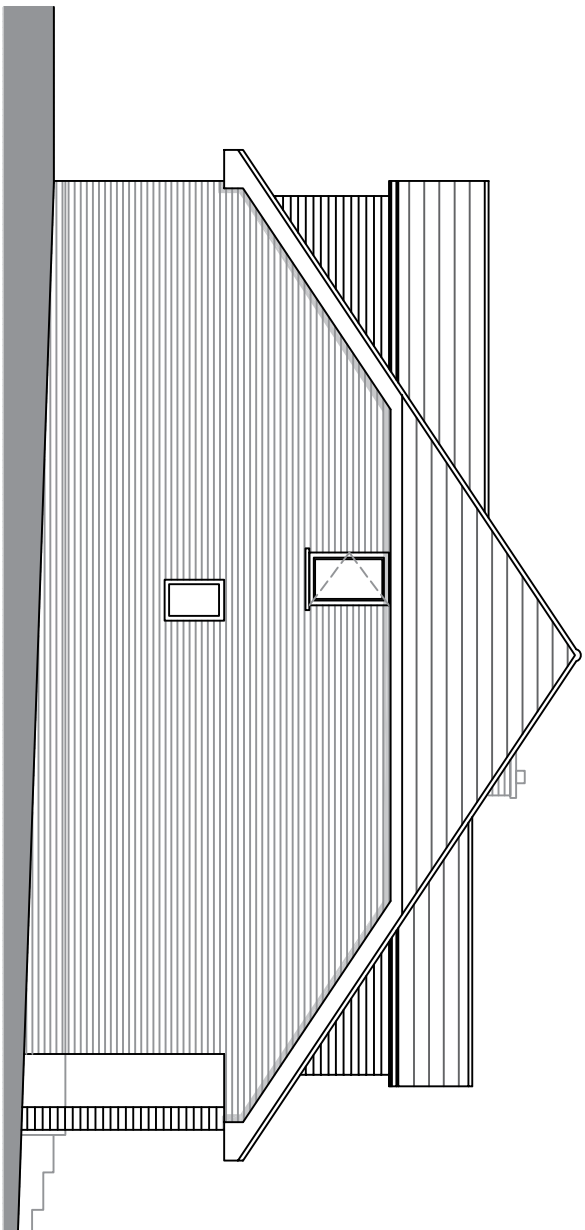
Proposed Side Elevation 1 : 100 @ A3
