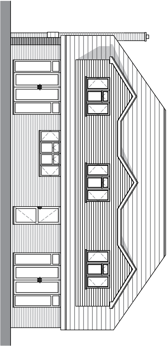
Proposed Rear Elevation 1 : 100 @ A3
