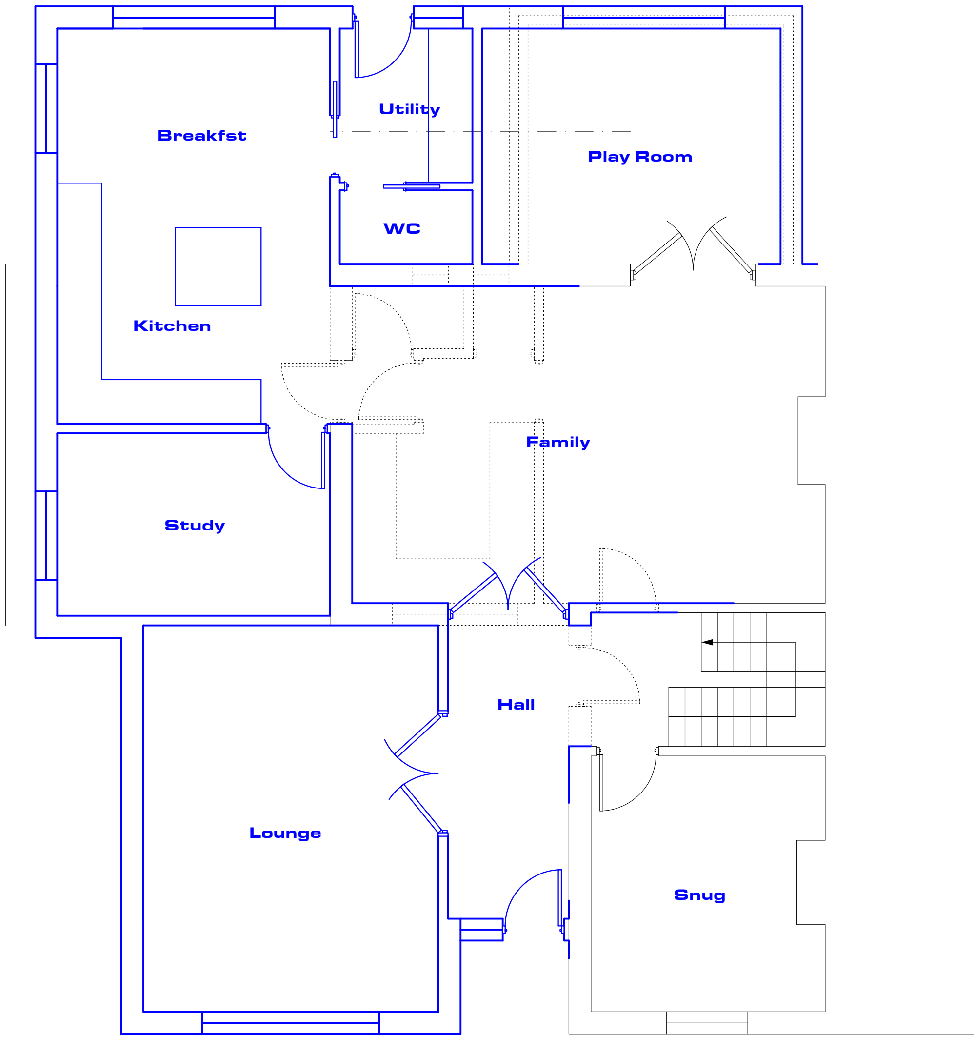
Proposed Ground Floor Plan 1:50 0 1 2 3 4 5m © MDT Design
