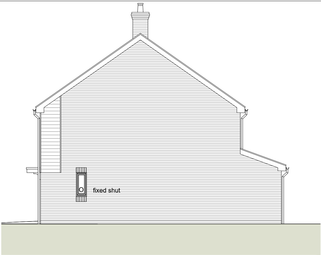
Side Elevation O= Obscure glazed window.
