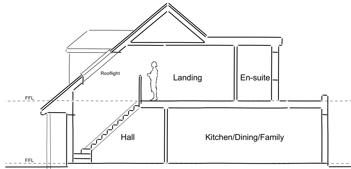
PROPOSED SECTION B
