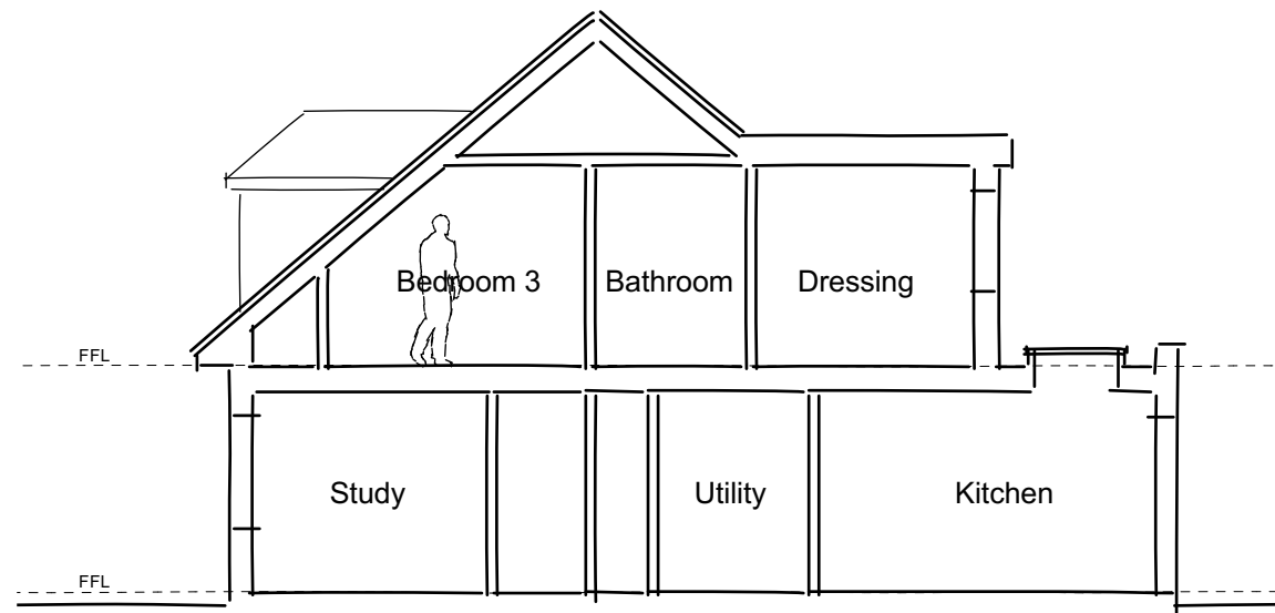
PROPOSED SECTION A
