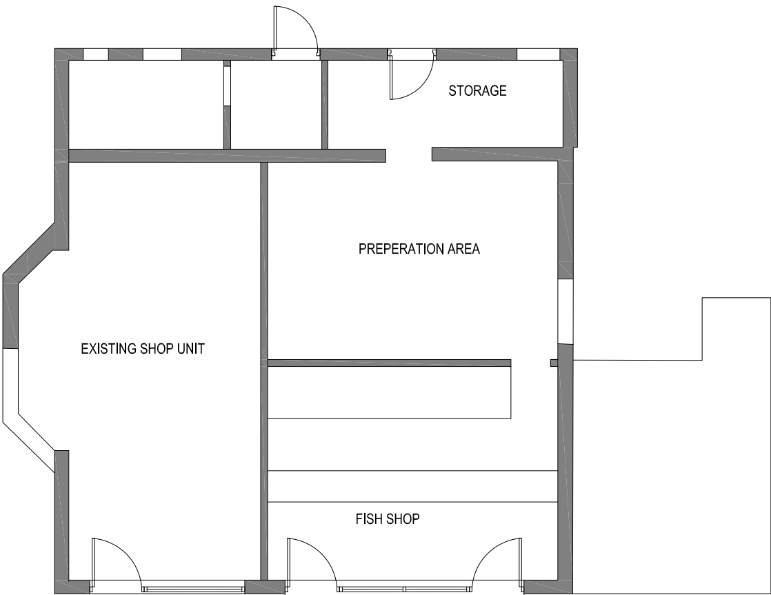
GROUND FLOOR
