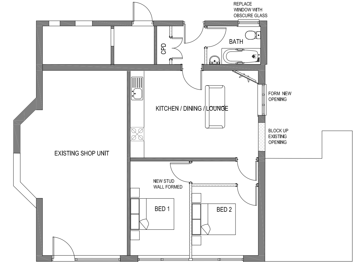
GROUND FLOOR
