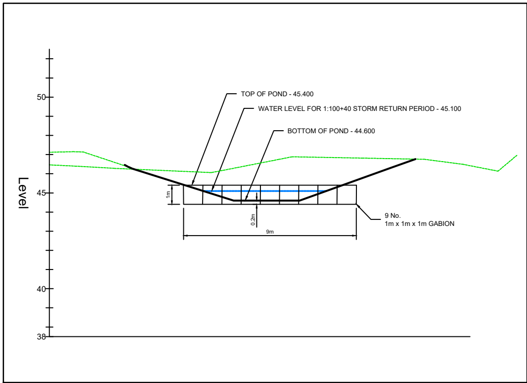
PROPOSED POND SECTION P2-P2
