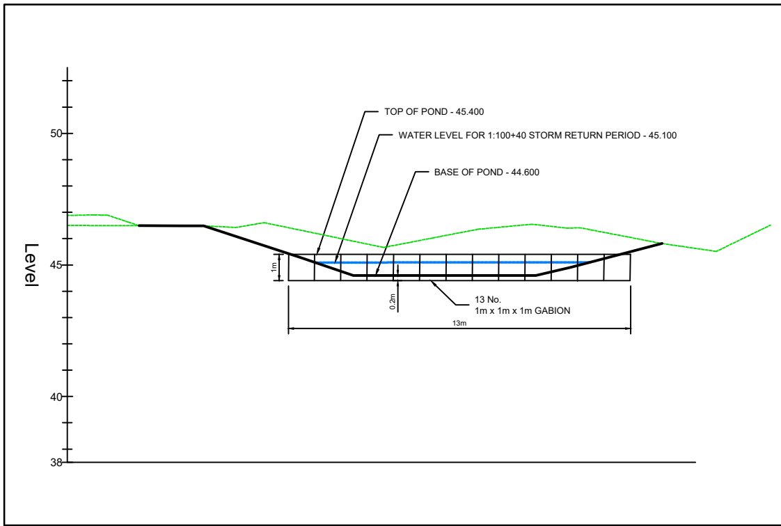
PROPOSED POND SECTION P3-P3
