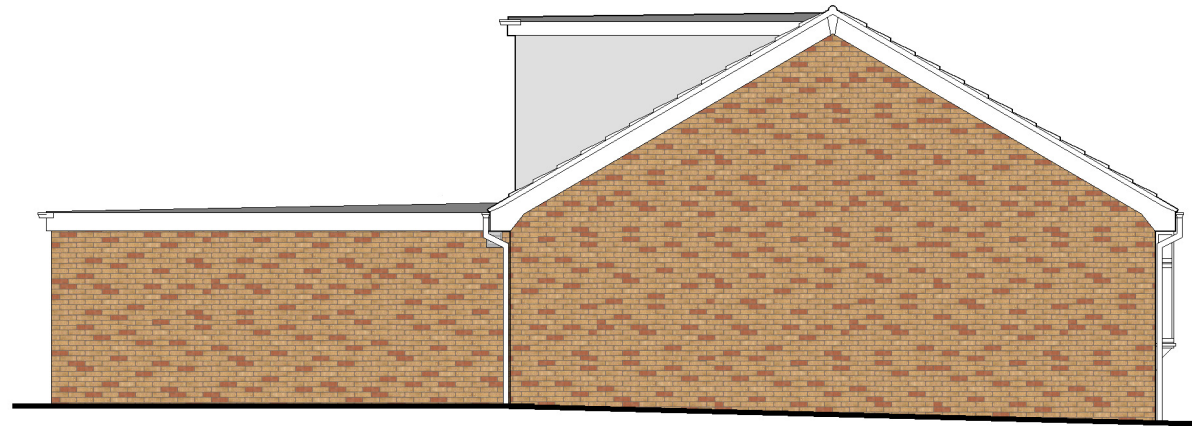
Side Elevation 1:100 (looking from 59 Haig Road)
